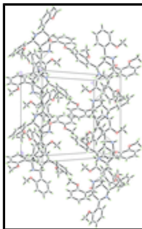
Fig. 2. The crystal packing of title compound, showing the molecules linked along the b axis. The solvent molecules are omitted for clarity. Intermolecular hydrogen bonds are shown as dashed lines.
